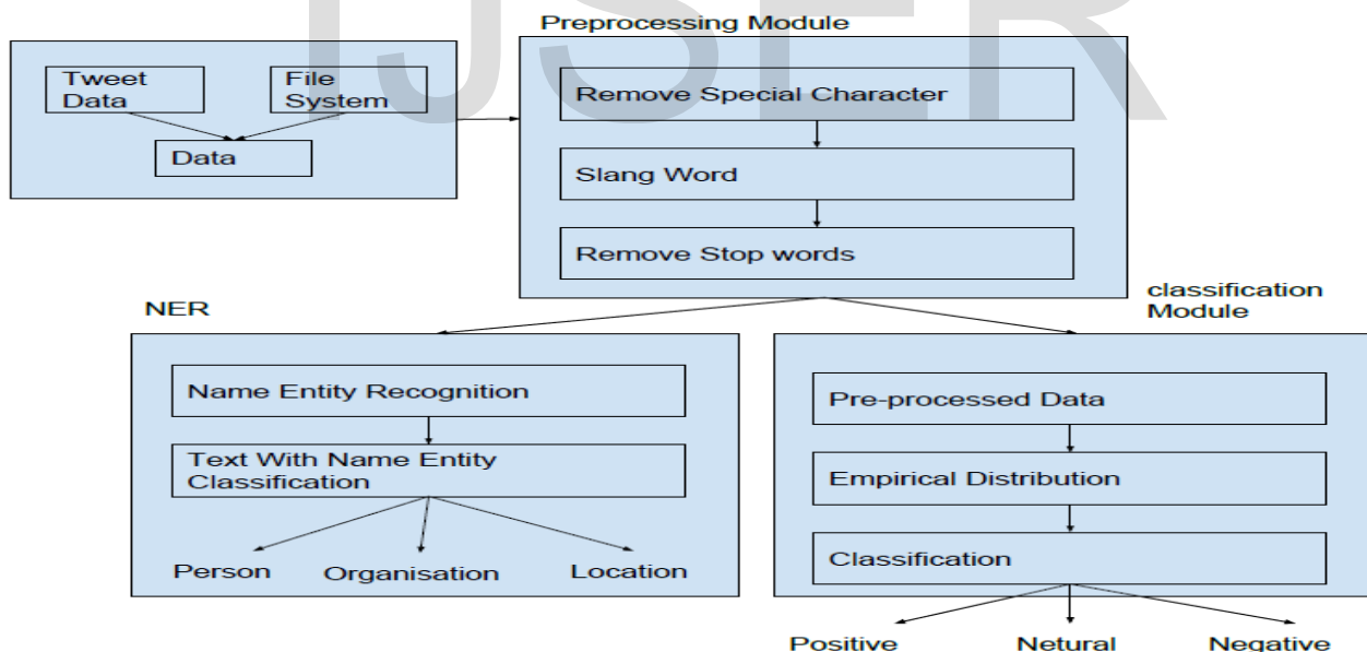
Fig. 1 Proposed Architecture of tweet data pre-processing and segmentation to NER.
